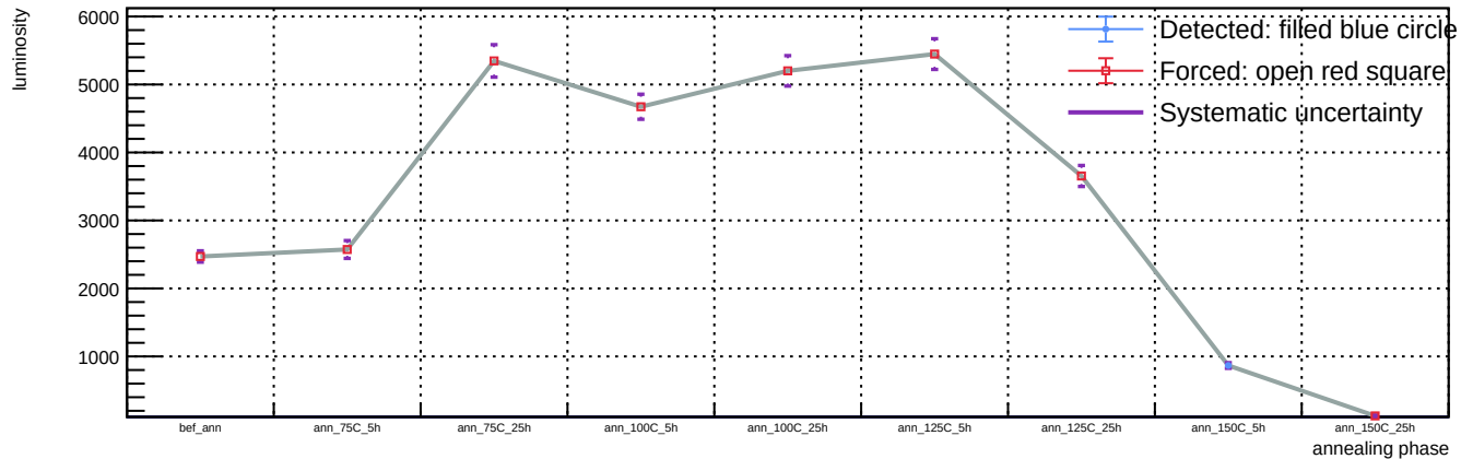
Sensor B1, T = 20 C, representative v = 55.9 V (max available) - Spot 114: luminosity vs phase
