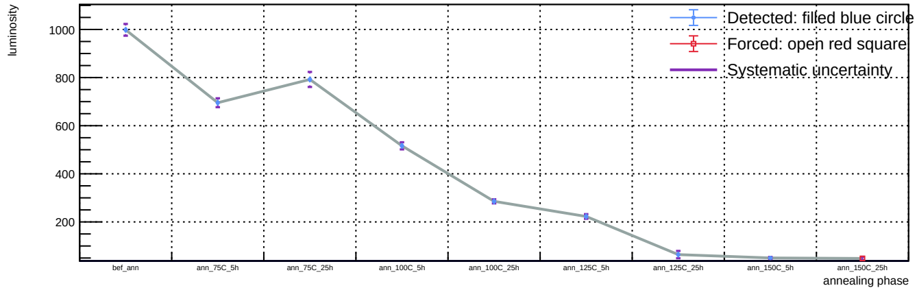
Sensor B1, T = 20 C, representative v = 55.9 V (max available) - Spot 18: luminosity vs phase
