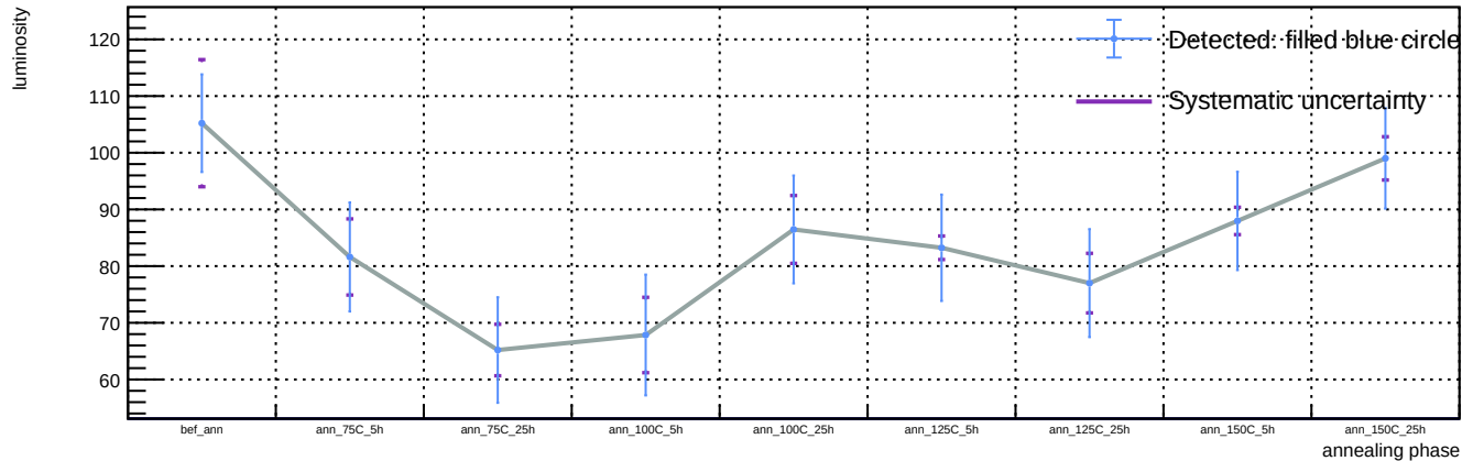
Sensor B1, T = 20 C, representative v = 55.9 V (max available) - Spot 21: luminosity vs phase
