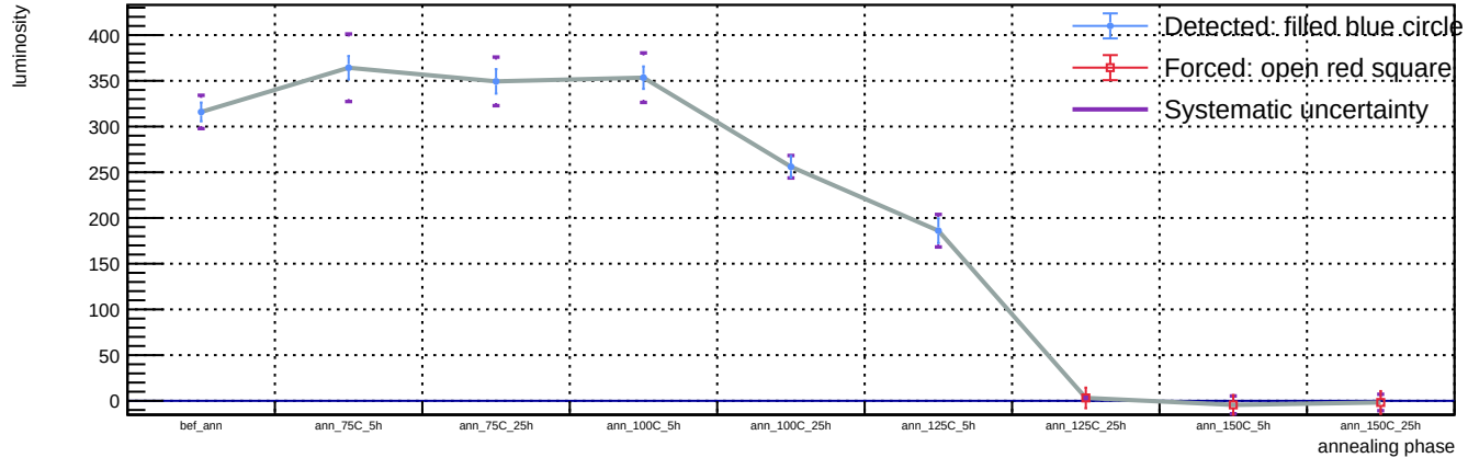
Sensor B1, T = 20 C, representative v = 55.9 V (max available) - Spot 22: luminosity vs phase
