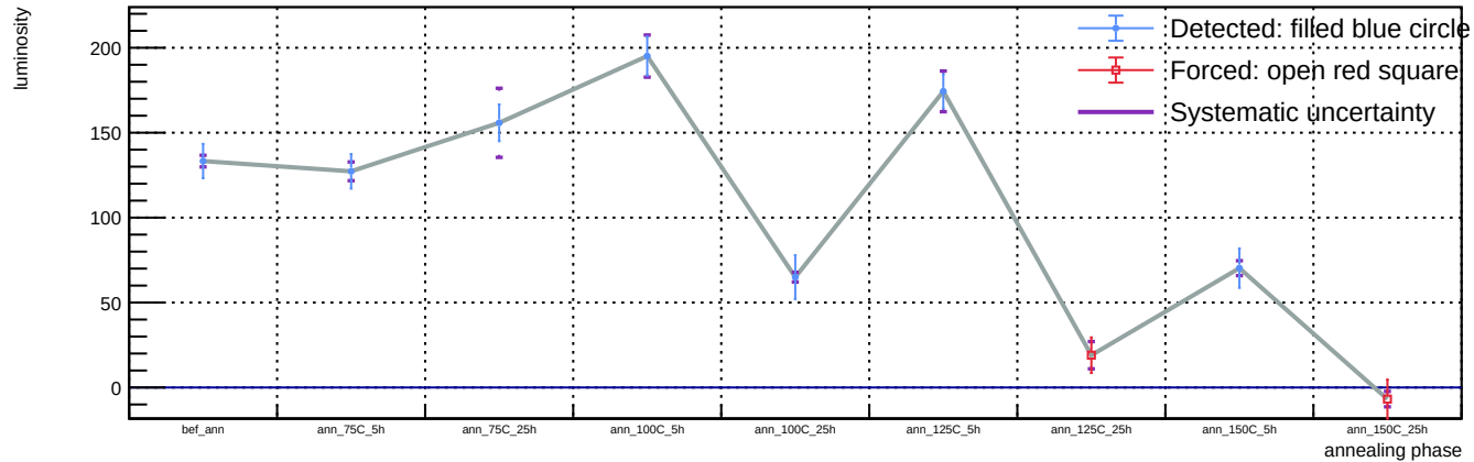
Sensor B1, T = 20 C, representative v = 55.9 V (max available) - Spot 27: luminosity vs phase
