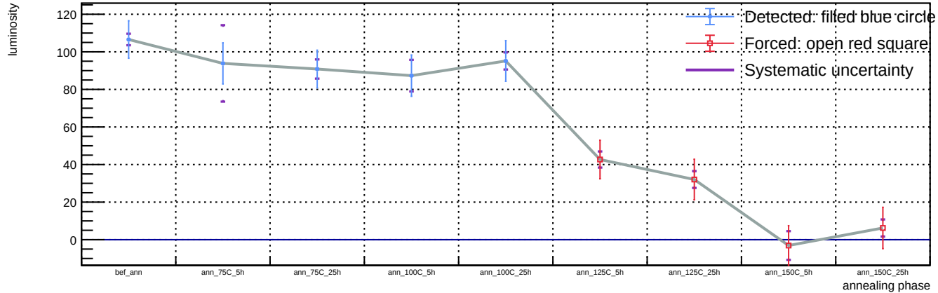
Sensor B1, T = 20 C, representative v = 55.9 V (max available) - Spot 3: luminosity vs phase
