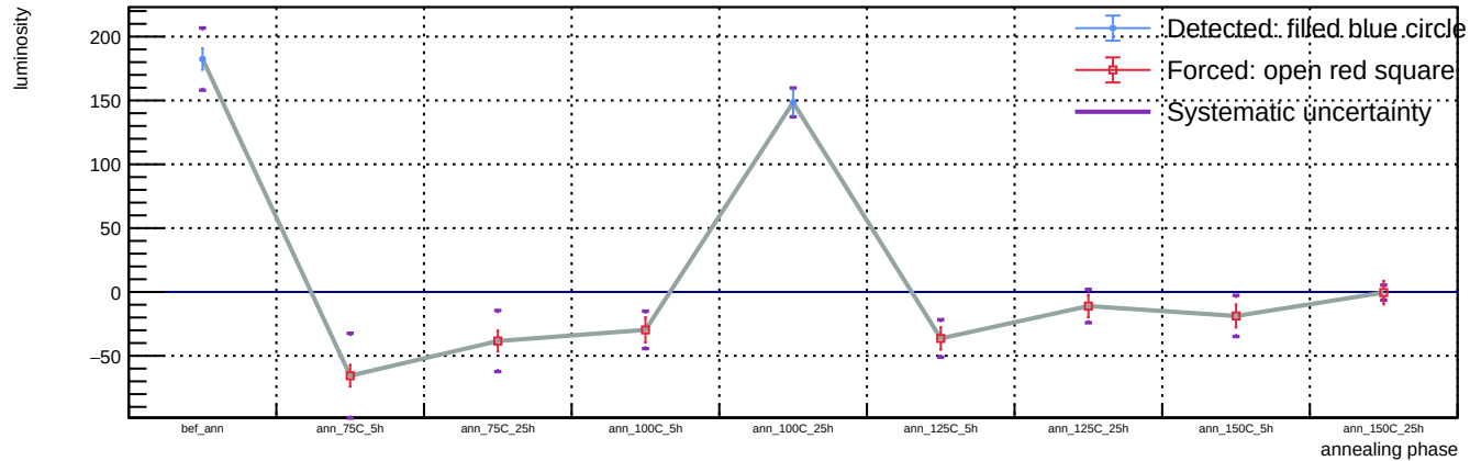
Sensor B1, T = 20 C, representative v = 55.9 V (max available) - Spot 35: luminosity vs phase
