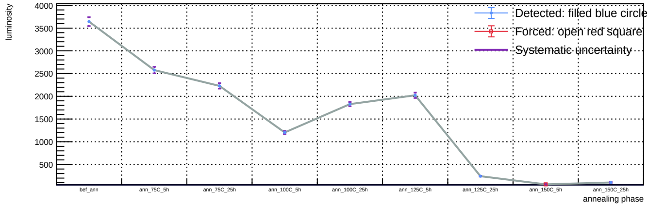
Sensor B1, T = 20 C, representative v = 55.9 V (max available) - Spot 36: luminosity vs phase
