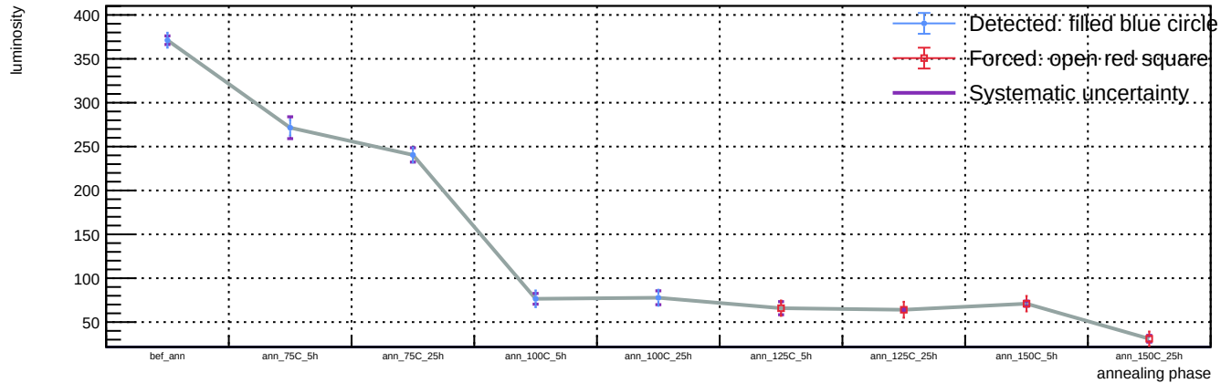
Sensor B1, T = 20 C, representative v = 55.9 V (max available) - Spot 39: luminosity vs phase
