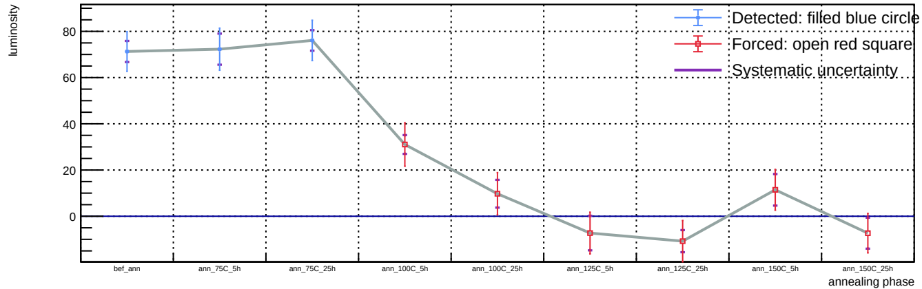
Sensor B1, T = 20 C, representative v = 55.9 V (max available) - Spot 41: luminosity vs phase
