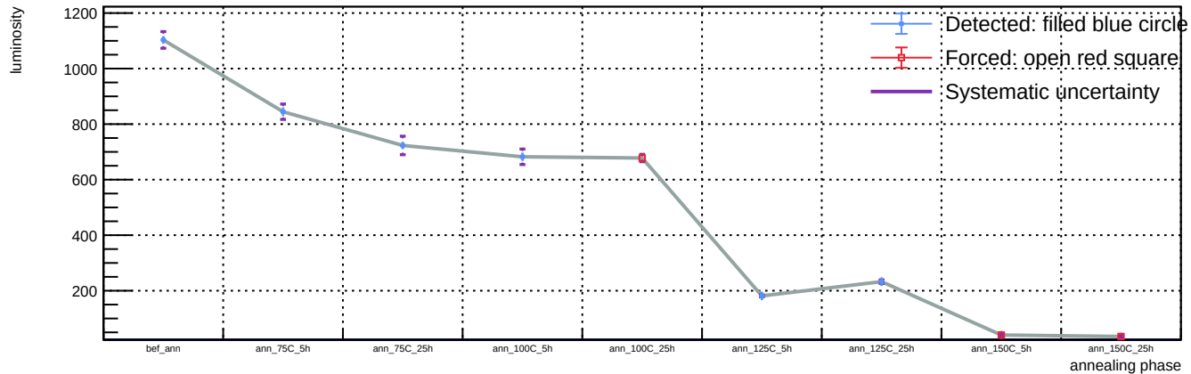
Sensor B1, T = 20 C, representative v = 55.9 V (max available) - Spot 42: luminosity vs phase
