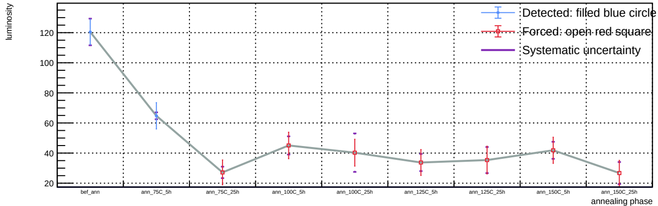
Sensor B1, T = 20 C, representative v = 55.9 V (max available) - Spot 44: luminosity vs phase
