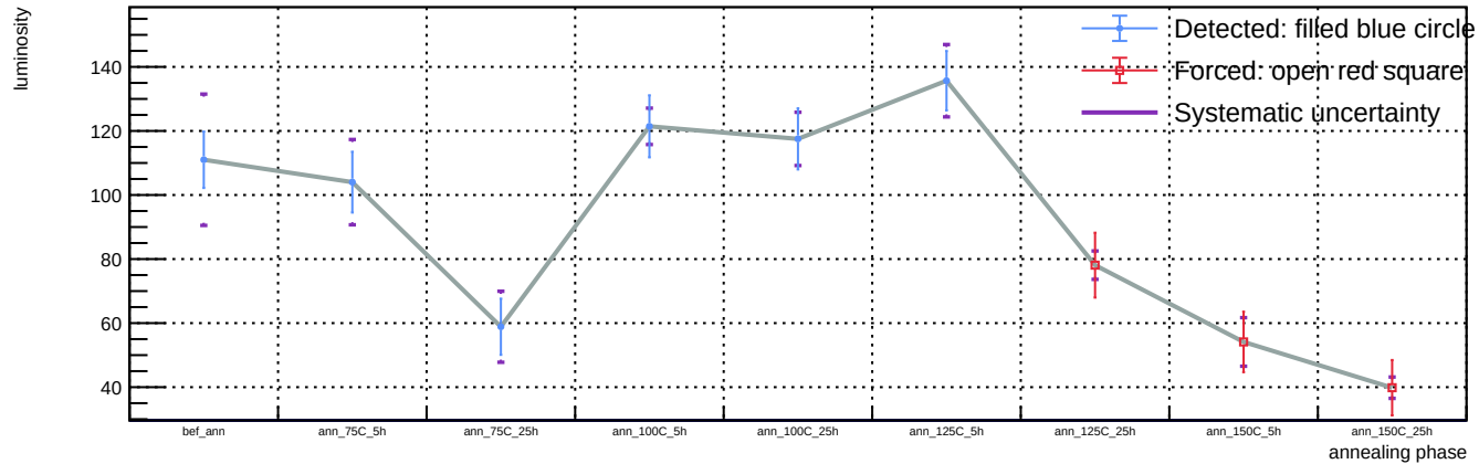
Sensor B1, T = 20 C, representative v = 55.9 V (max available) - Spot 46: luminosity vs phase
