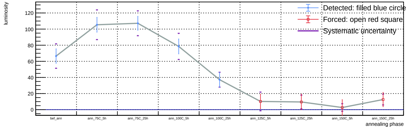
Sensor B1, T = 20 C, representative v = 55.9 V (max available) - Spot 47: luminosity vs phase
