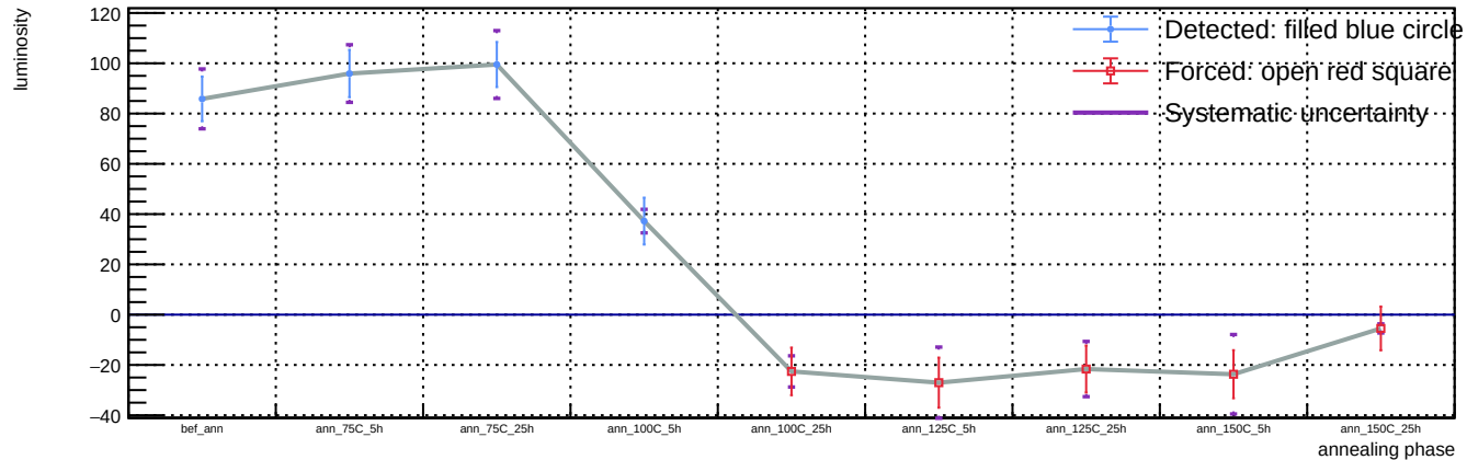
Sensor B1, T = 20 C, representative v = 55.9 V (max available) - Spot 49: luminosity vs phase
