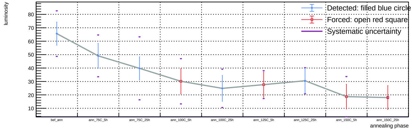
Sensor B1, T = 20 C, representative v = 55.9 V (max available) - Spot 51: luminosity vs phase
