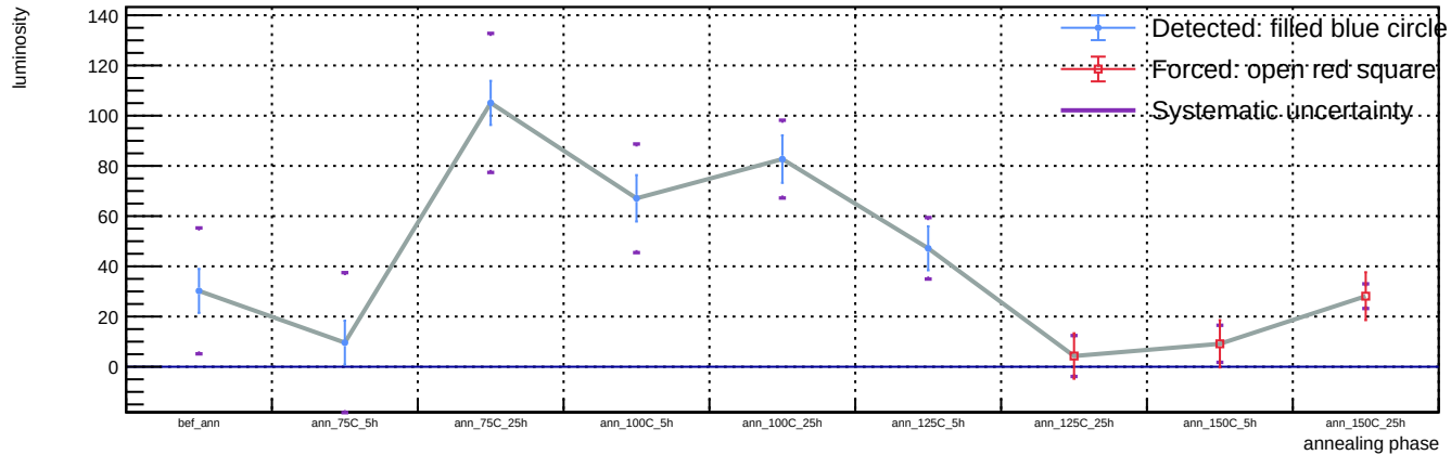
Sensor B1, T = 20 C, representative v = 55.9 V (max available) - Spot 54: luminosity vs phase
