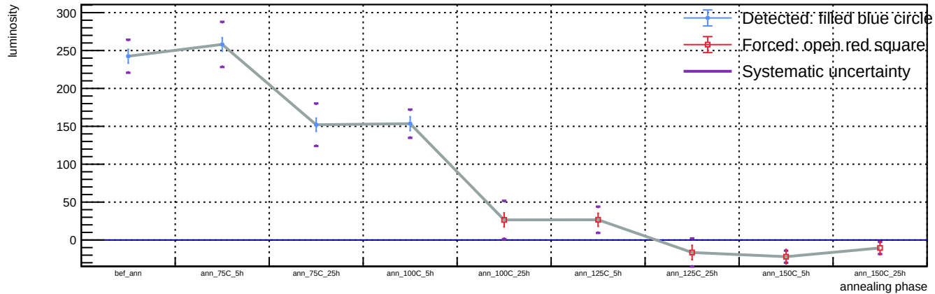
Sensor B1, T = 20 C, representative v = 55.9 V (max available) - Spot 55: luminosity vs phase
