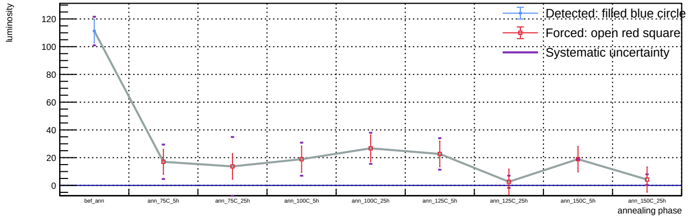
Sensor B1, T = 20 C, representative v = 55.9 V (max available) - Spot 57: luminosity vs phase
