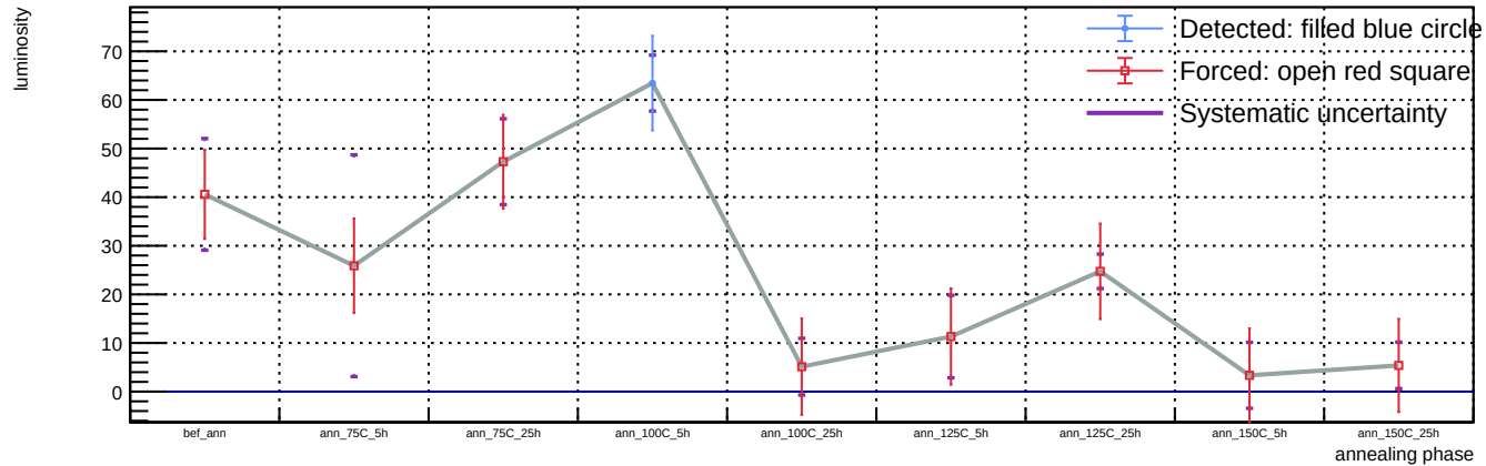
Sensor B1, T = 20 C, representative v = 55.9 V (max available) - Spot 62: luminosity vs phase
