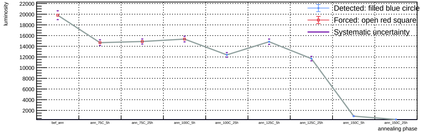
Sensor B1, T = 20 C, representative v = 55.9 V (max available) - Spot 63: luminosity vs phase
