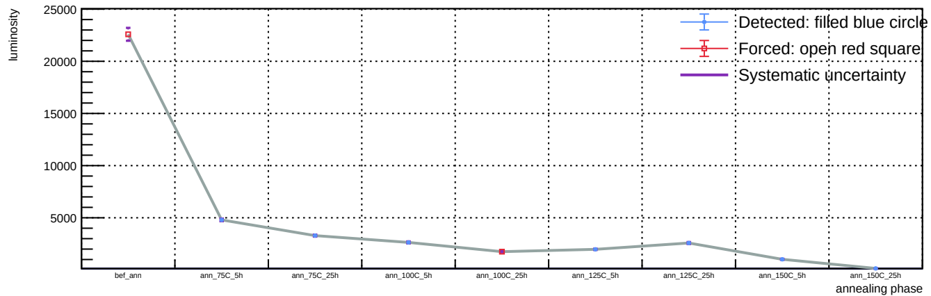
Sensor B1, T = 20 C, representative v = 55.9 V (max available) - Spot 65: luminosity vs phase
