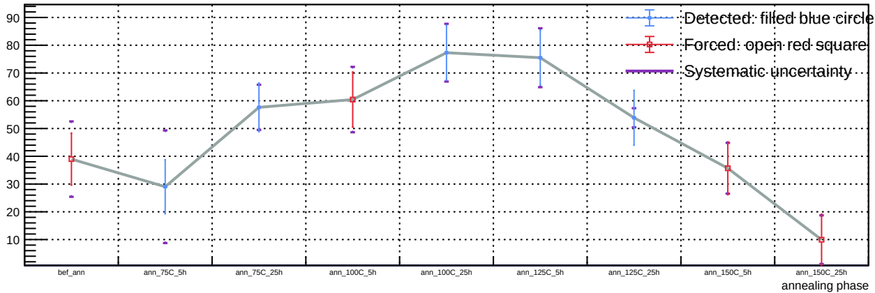
Sensor B1, T = 20 C, representative v = 55.9 V (max available) - Spot 68: luminosity vs phase
