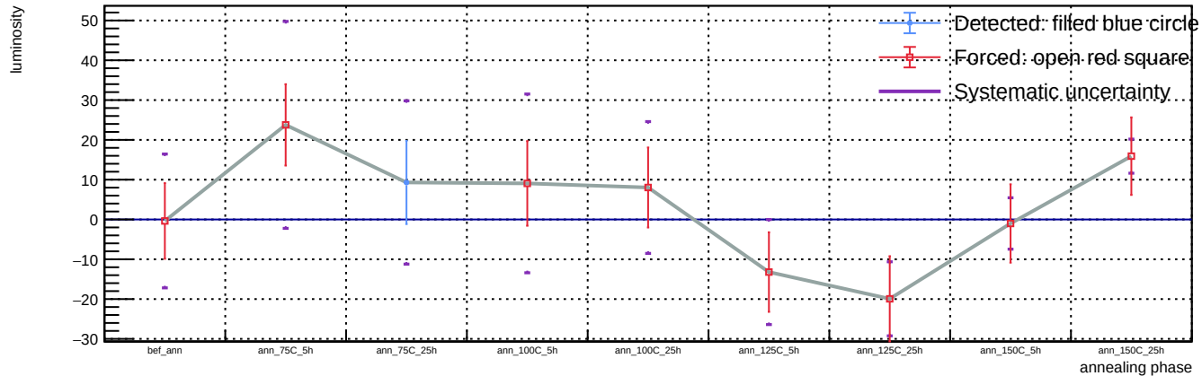
Sensor B1, T = 20 C, representative v = 55.9 V (max available) - Spot 69: luminosity vs phase
