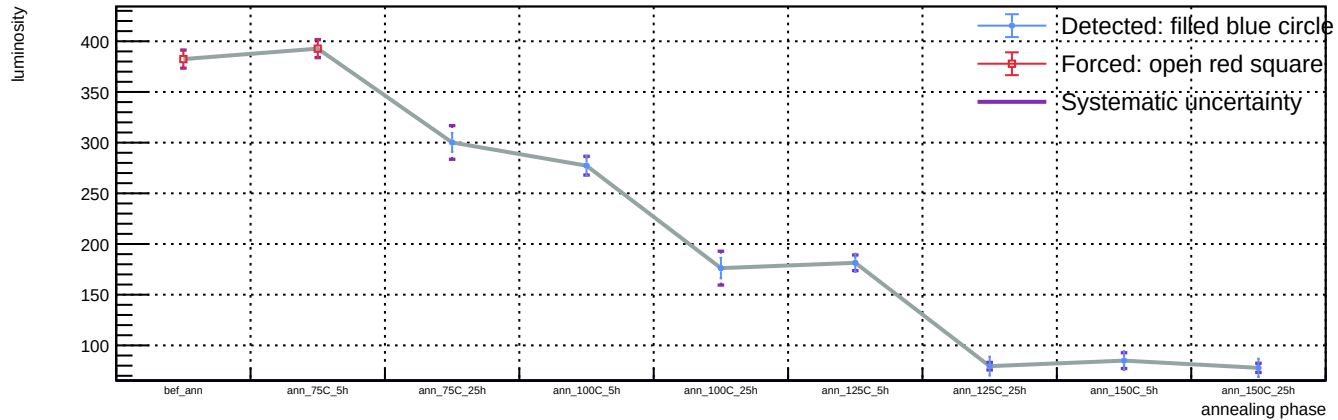
Sensor B1, T = 20 C, representative v = 55.9 V (max available) - Spot 74: luminosity vs phase
