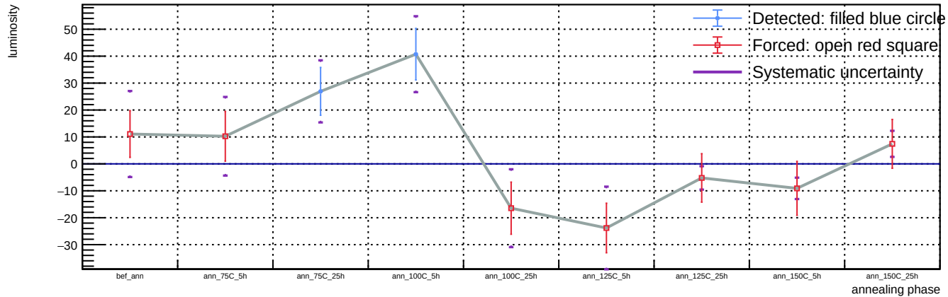
Sensor B1, T = 20 C, representative v = 55.9 V (max available) - Spot 75: luminosity vs phase
