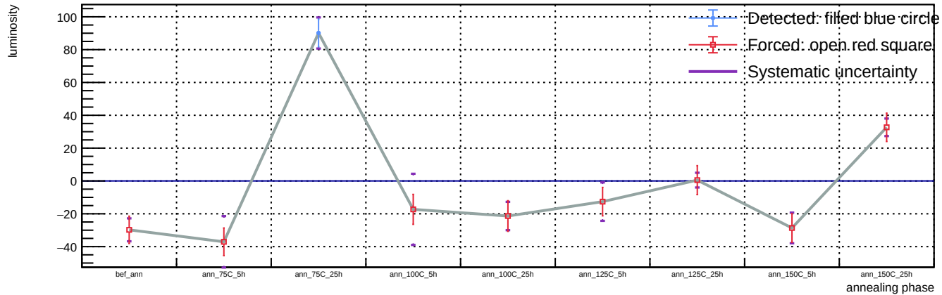
Sensor B1, T = 20 C, representative v = 55.9 V (max available) - Spot 77: luminosity vs phase
