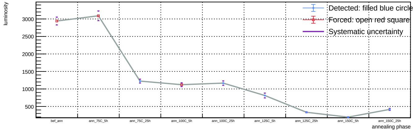
Sensor B1, T = 20 C, representative v = 55.9 V (max available) - Spot 78: luminosity vs phase
