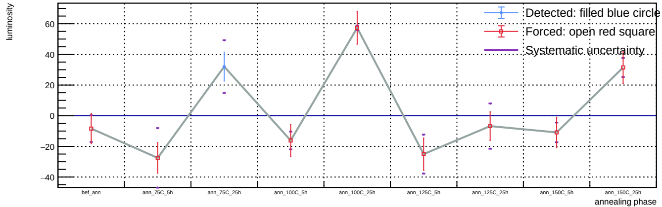
Sensor B1, T = 20 C, representative v = 55.9 V (max available) - Spot 79: luminosity vs phase
