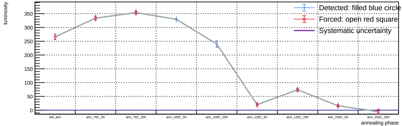
Sensor B1, T = 20 C, representative v = 55.9 V (max available) - Spot 80: luminosity vs phase
