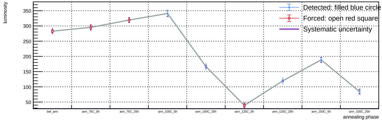
Sensor B1, T = 20 C, representative v = 55.9 V (max available) - Spot 83: luminosity vs phase
