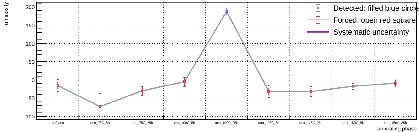
Sensor B1, T = 20 C, representative v = 55.9 V (max available) - Spot 86: luminosity vs phase
