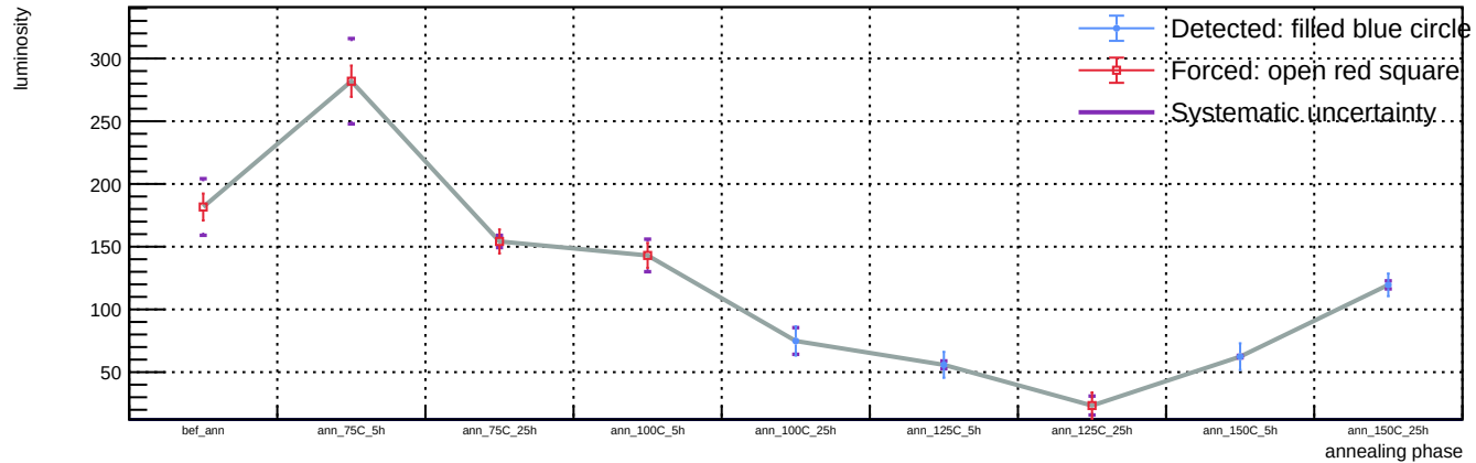
Sensor B1, T = 20 C, representative v = 55.9 V (max available) - Spot 88: luminosity vs phase
