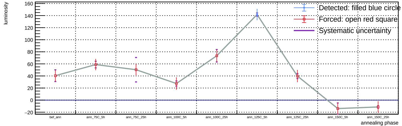
Sensor B1, T = 20 C, representative v = 55.9 V (max available) - Spot 97: luminosity vs phase
