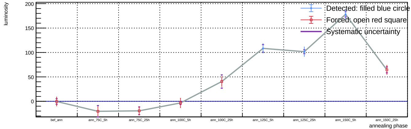
Sensor B1, T = 20 C, representative v = 55.9 V (max available) - Spot 98: luminosity vs phase
