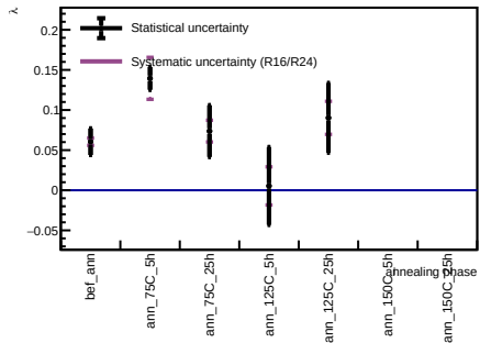
Sensor B1, v = 3 V - Spot 10
