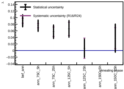
Sensor B1, v = 3 V - Spot 6
