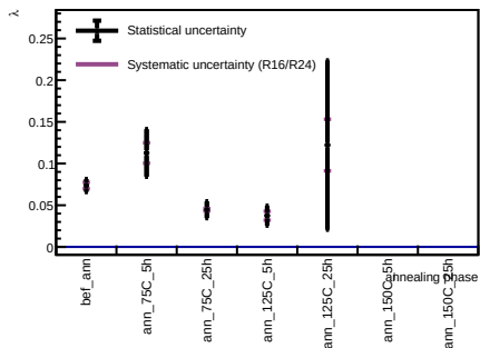
Sensor B1, v = 3 V - Spot 40
