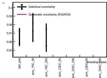
Sensor B1, v = 3 V - Spot 39
