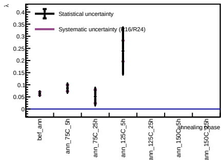
Sensor B1, v = 3 V - Spot 37
