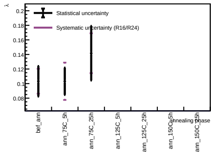
Sensor B1, v = 3 V - Spot 55
