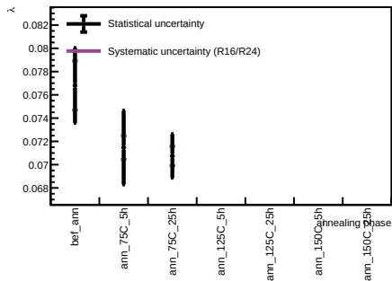
Sensor B1, v = 3 V - Spot 59
