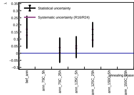
Sensor B1, v = 3 V - Spot 68
