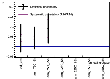
Sensor B1, v = 3 V - Spot 67
