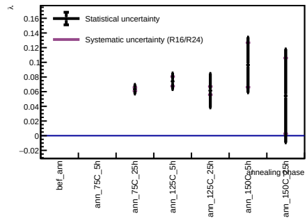
Sensor B1, v = 3 V - Spot 78
