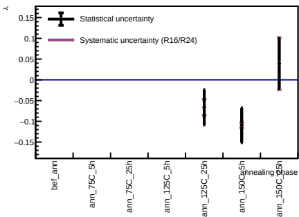
Sensor B1, v = 3 V - Spot 105
