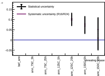
Sensor B1, v = 3 V - Spot 106
