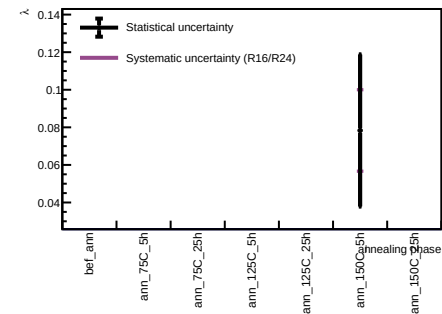
Sensor B1, v = 3 V - Spot 113
