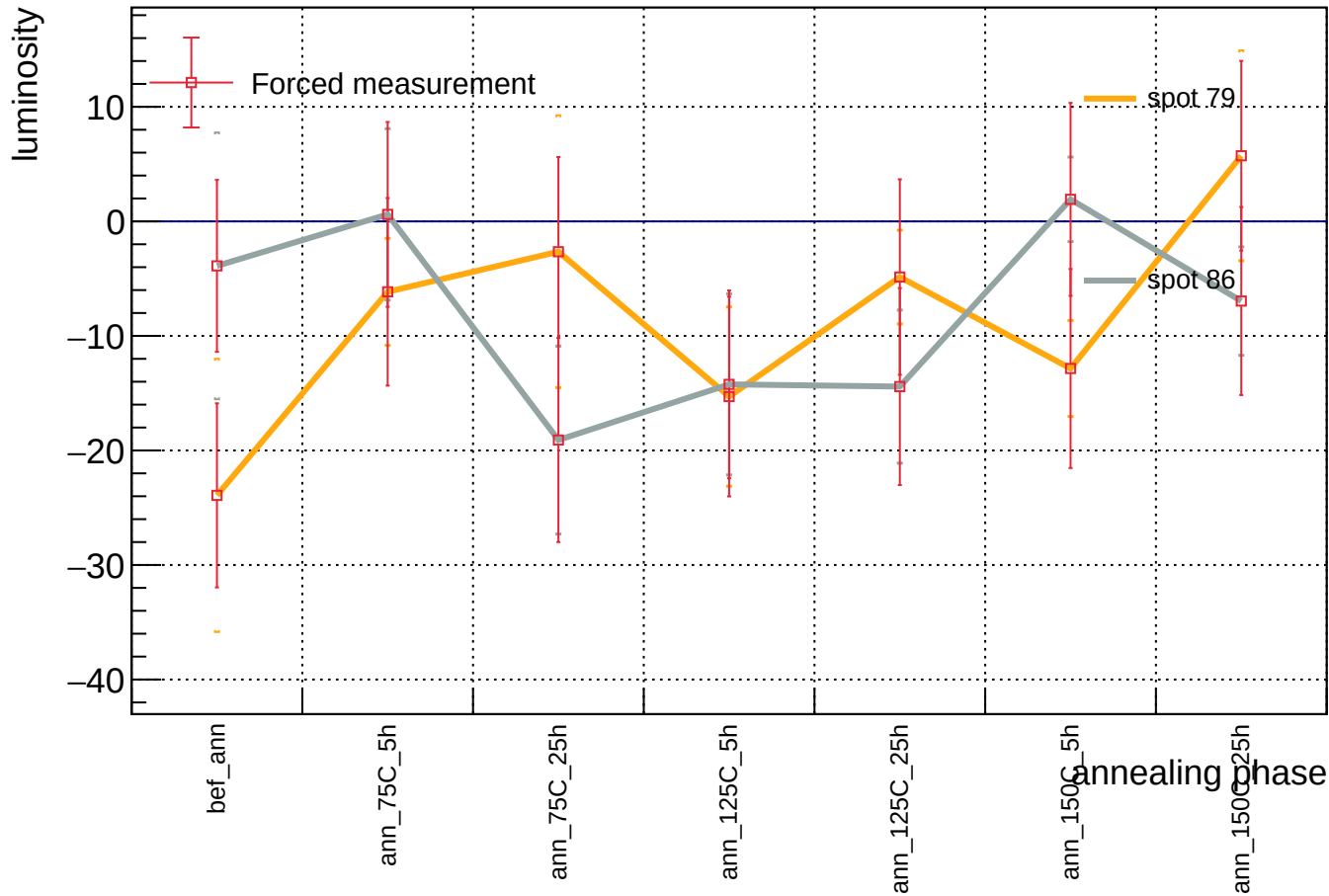
Sensor B1, v = 3 V, representative T = 23 C (max available) - luminosity vs phase - order 10^0
