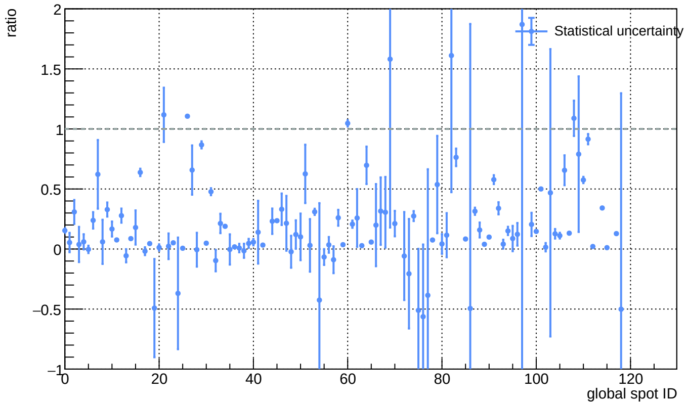
Sensor B1, v = 3 V - L(\text{ann\_150C\_5h}) / L(\text{before\_annealing})
