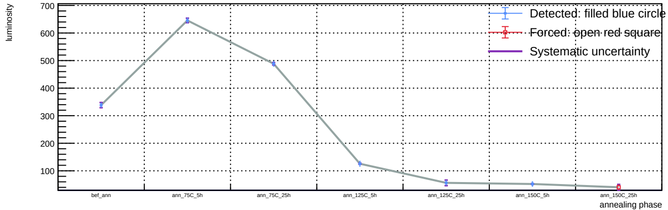
Sensor B1, v = 3 V, representative T = 23 C (max available) - Spot 0: luminosity vs phase
