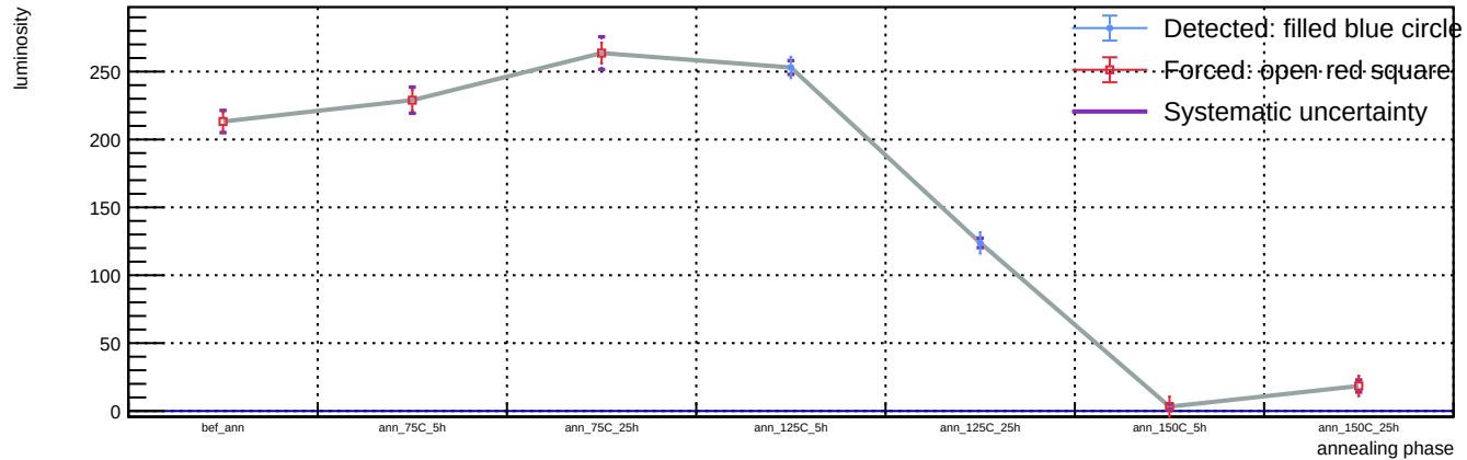
Sensor B1, v = 3 V, representative T = 23 C (max available) - Spot 102: luminosity vs phase
