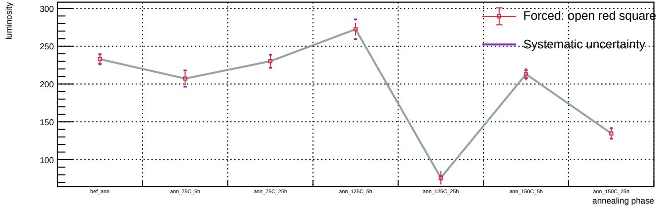
Sensor B1, v = 3 V, representative T = 23 C (max available) - Spot 111: luminosity vs phase
