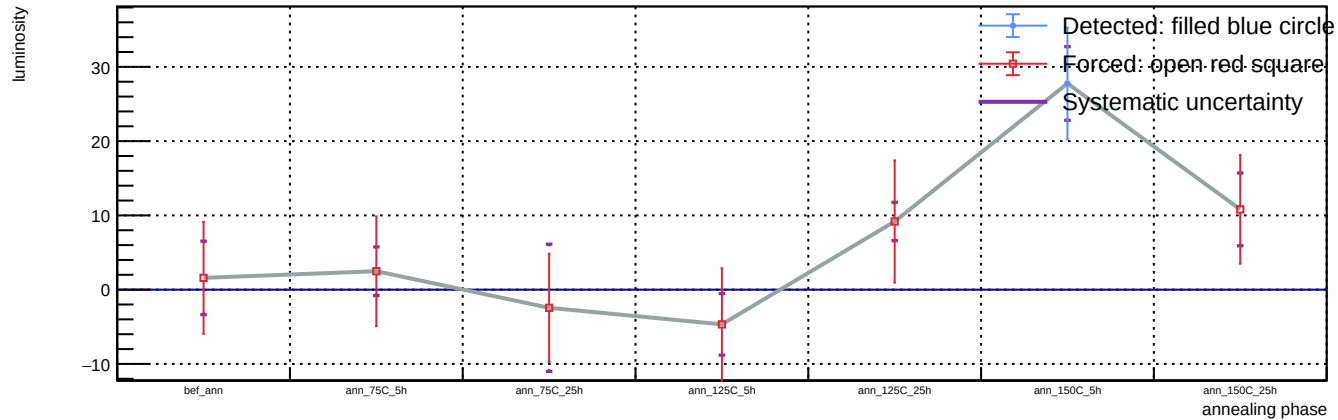
Sensor B1, v = 3 V, representative T = 23 C (max available) - Spot 116: luminosity vs phase
