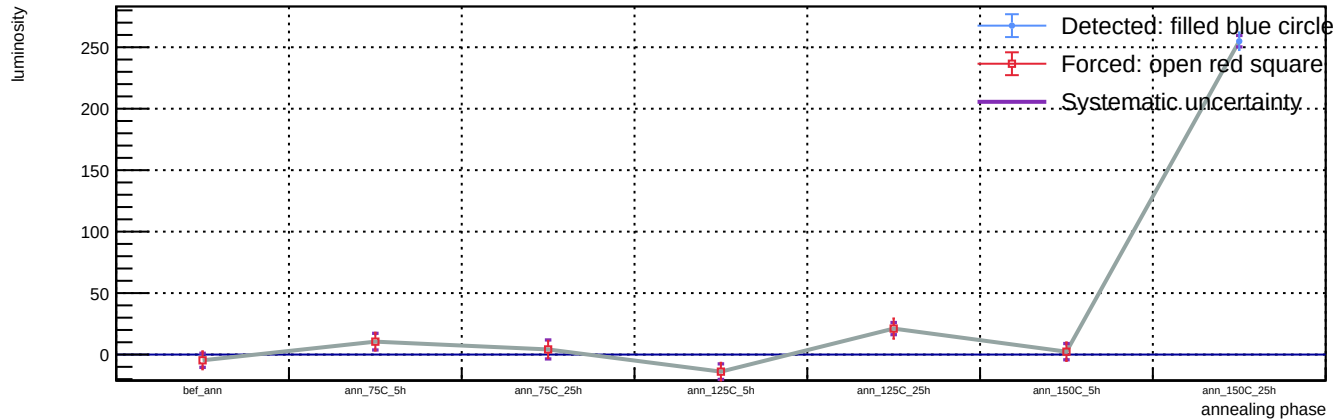
Sensor B1, v = 3 V, representative T = 23 C (max available) - Spot 118: luminosity vs phase
