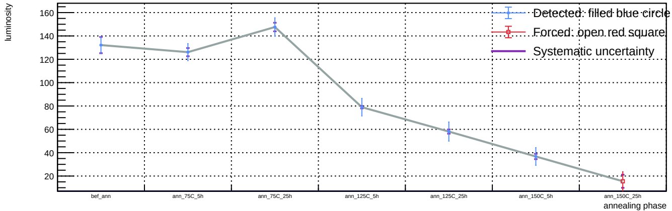
Sensor B1, v = 3 V, representative T = 23 C (max available) - Spot 12: luminosity vs phase
